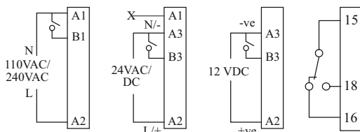
11RDT4, 12RDT4, 15DDT4
