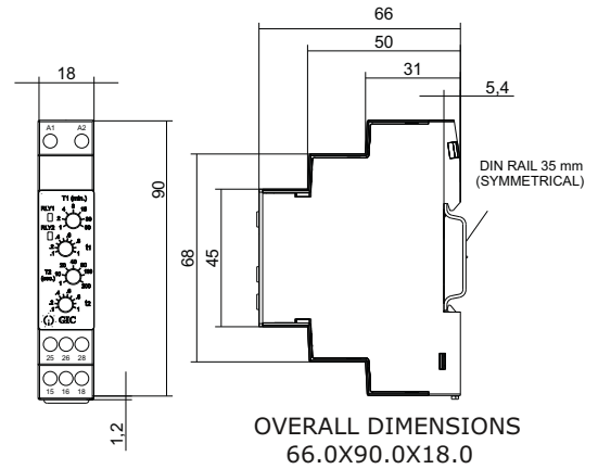
All Dimensions are in mm 1CMDT0, 1CQDT9, 1CJDT0, 1CMDTF, 1CZDTF STAIRCASE TIMER 11WDT, 12WDT
